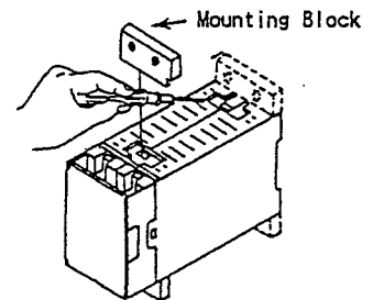
Fig.4 Installation and removal of Mounting Block
