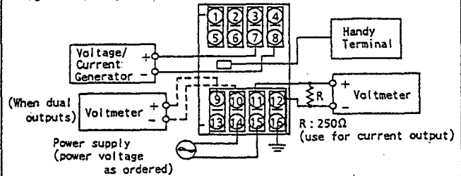
Fig.10 Wiring of Calibration Equipment
