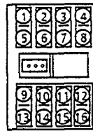
Fig.8 Terminal Arrangement
