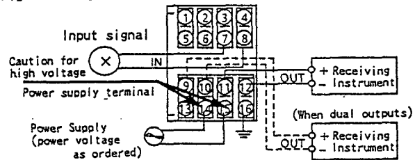
Fig.10 Wiring of Calibration Equipment
