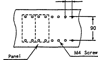
Fig.8 Terminal Arrangement
